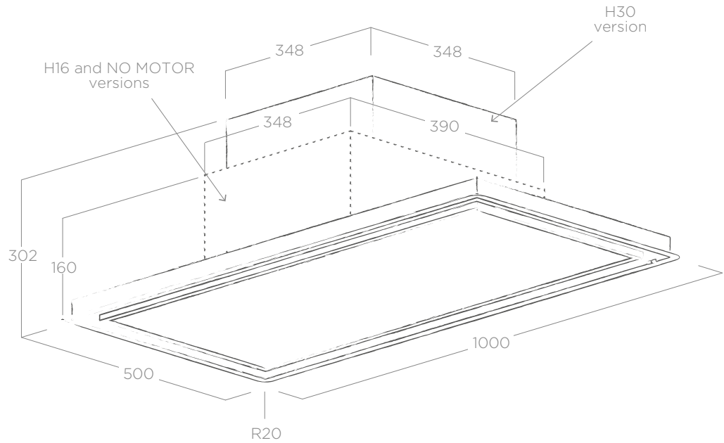
FALSE CEILING CUT: 480X980
