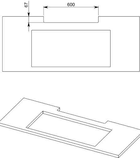
Foro top per inserimento K-MAGNETOLAB Hole on the top to place K-MAGNETOLAB
