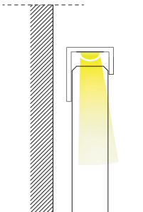
ILLUMINAZIONE LED INTEGRATA BUILT-IN LED LIGHTING
